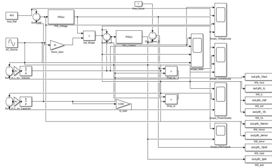
Fig. 2. Simulink implementation of the averaged boost PFC model, showing the dual-loop control architecture, the averaged plant dynamics, and the scope groups used for logging the simulation results.
