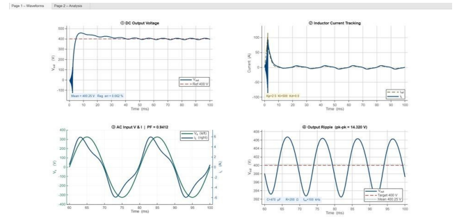
Fig. 3. Simulation waveform results from the averaged PFC model: DC output voltage, inductor current tracking, AC input voltage and output ripple around the 400 V reference.
